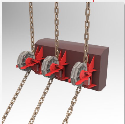
Underwater fairlead
